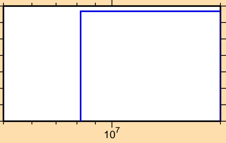
\sigma vs. E for ^{150}\text{Ho}(n,\text{pt})
