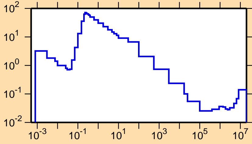
\sigma vs. E for ^{150}\text{Ho}(n,\alpha)
