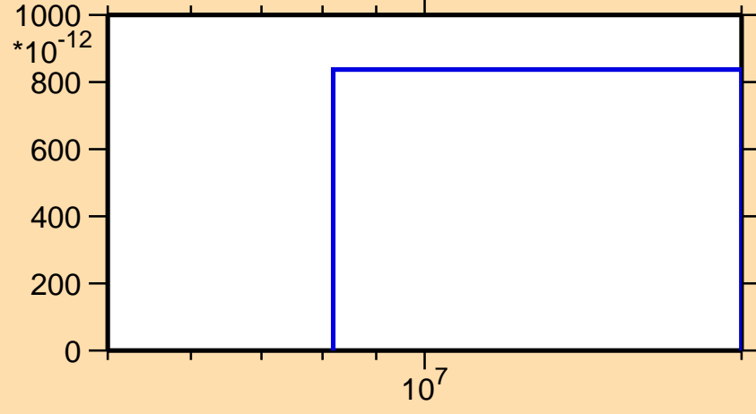
\sigma vs. E for ^{150}\text{Ho}(\text{mt } 34)
