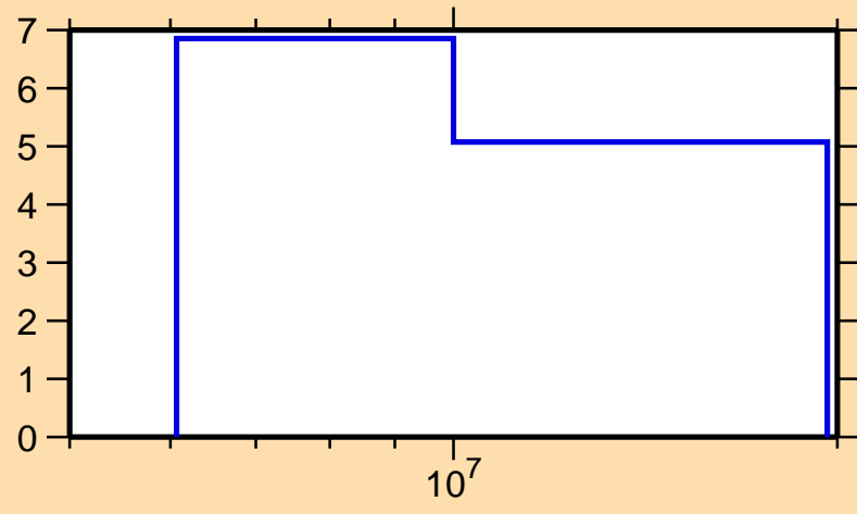
\Delta\sigma/\sigma vs. E for ^{151}\text{Ho}(n,\text{el.})
