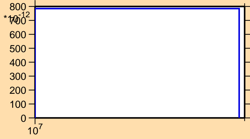
\sigma vs. E for ^{151}\text{Ho}(n,\text{pt})
