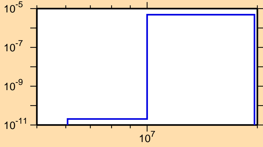
\sigma vs. E for ^{151}\text{Ho}(n,\text{He3})
