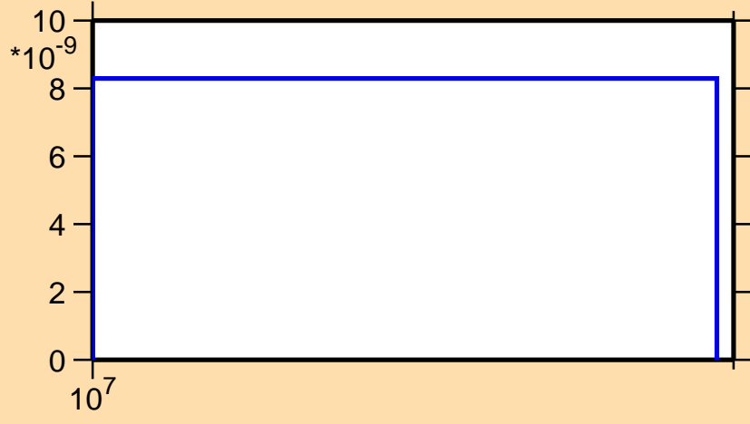
\sigma vs. E for ^{151}\text{Ho}(n,nt)
