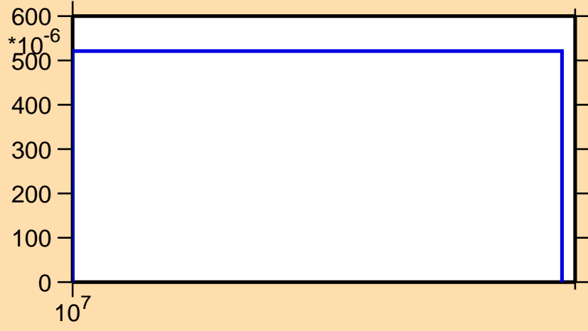
\sigma vs. E for ^{151}\text{Ho}(n,2np)
