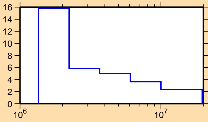
\Delta\sigma/\sigma vs. E for ^{151}\text{Ho}(n,\text{nonel.})
