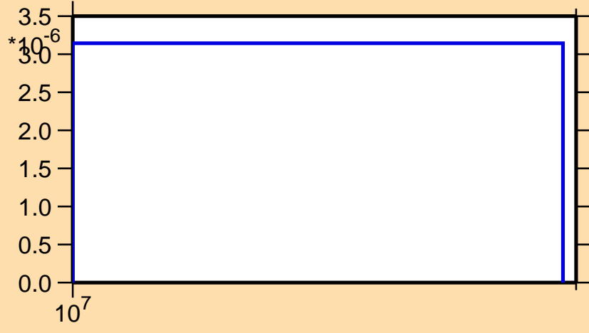
\sigma vs. E for ^{151}\text{Ho}(n,3n)
