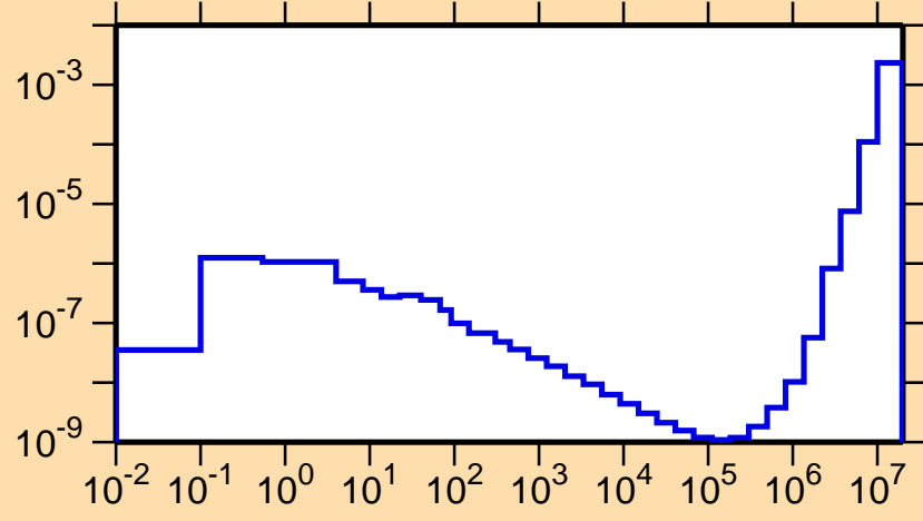
\sigma vs. E for ^{151}\text{Ho}(n,p\alpha)
