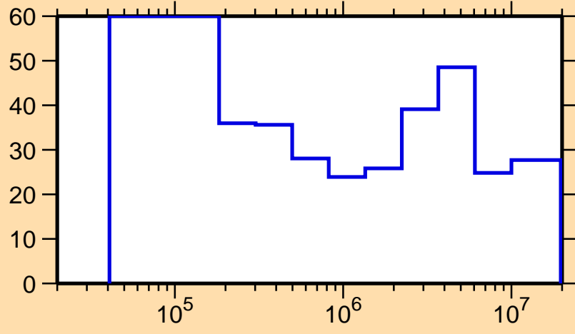
\Delta\sigma/\sigma vs. E for ^{151}\text{Ho}(n,n_1)
