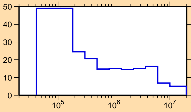
\Delta\sigma/\sigma vs. E for ^{151}\text{Ho}(n,\text{el.})
