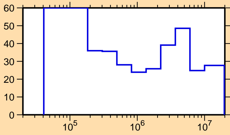
\Delta\sigma/\sigma vs. E for ^{151}\text{Ho}(n,n_1)
