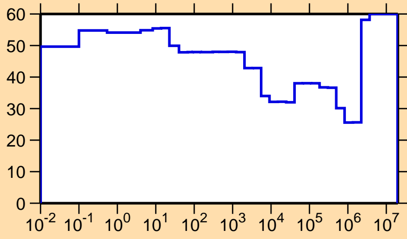
\Delta\sigma/\sigma vs. E for ^{151}\text{Ho}(n,p)
