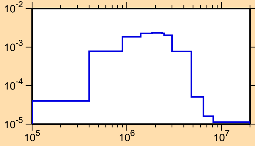
\sigma vs. E for ^{151}\text{Ho}(n,n_1)
