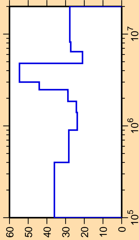
\Delta\sigma/\sigma vs. E for ^{151}\text{Ho}(n,n_1)
