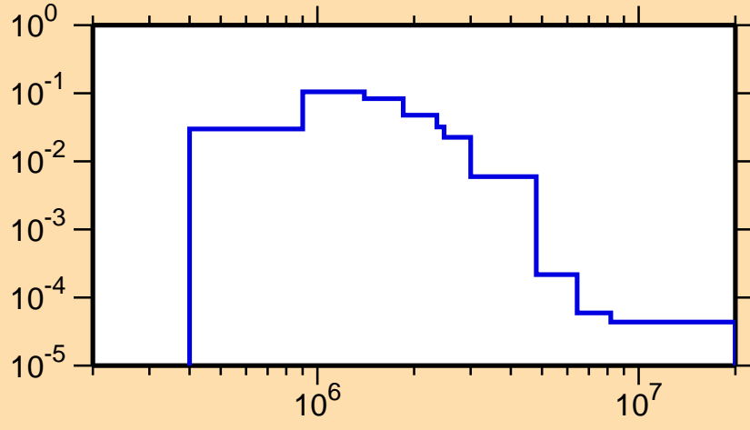
\sigma vs. E for ^{151}\text{Ho}(n,n_4)
