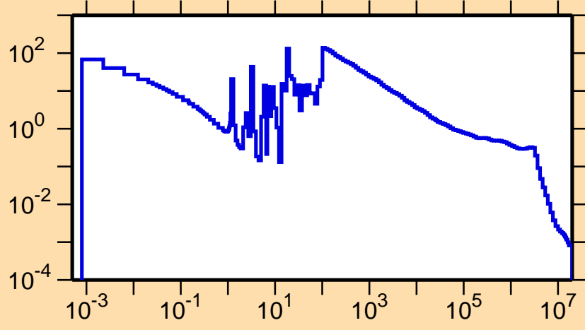
\sigma vs. E for ^{151}\text{Ho}(n,\gamma)
