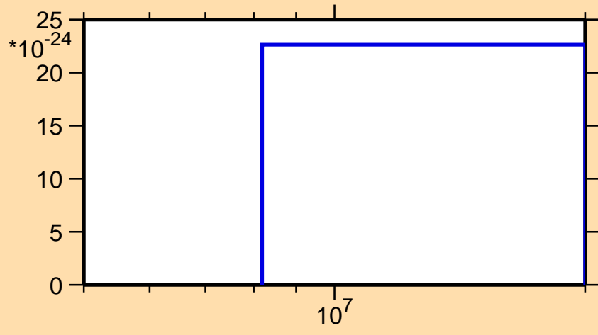
\sigma vs. E for ^{151}\text{Ho} (mt 42)
