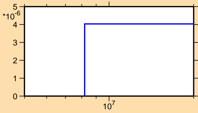
\sigma vs. E for ^{151}\text{Ho}(n,\text{nd})
