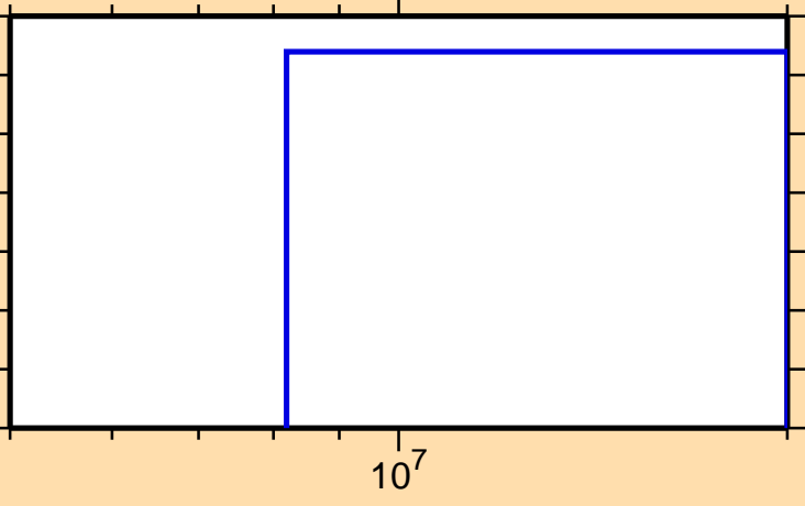
\sigma vs. E for ^{151}\text{Ho}(n,\text{pt})
