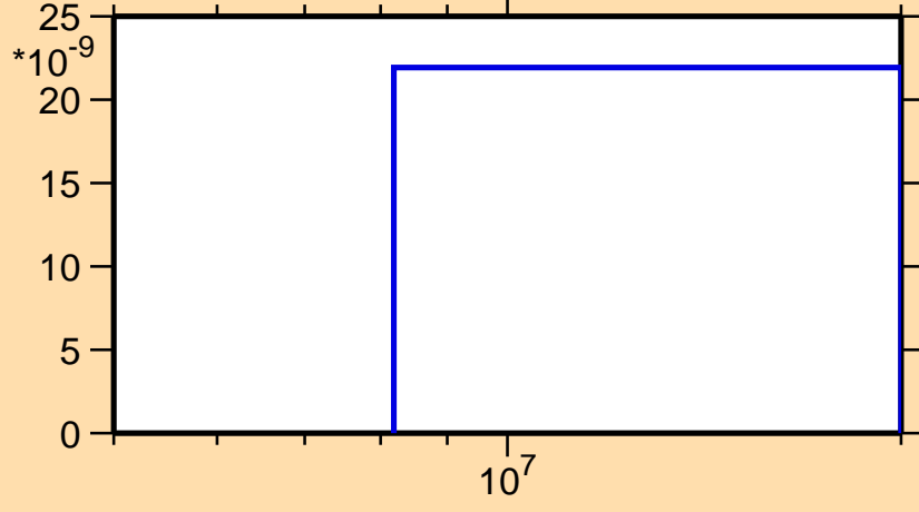
\sigma vs. E for ^{151}\text{Ho}(n,nt)
