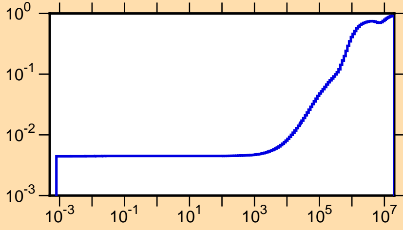
\mu vs. E for ^{152}\text{Ho}(\text{mt251})
