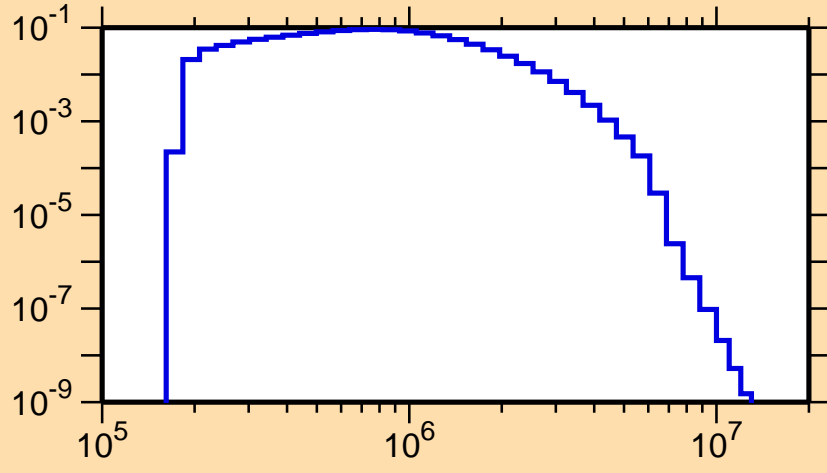
\sigma vs. E for ^{152}\text{Ho}(n,n_2)
