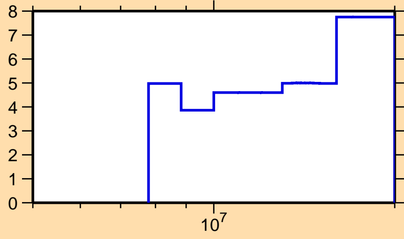
\Delta\sigma/\sigma vs. E for ^{152}\text{Ho}(n,\text{el.})
