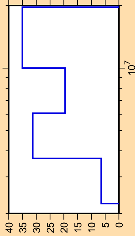
\Delta\sigma/\sigma vs. E for ^{152}\text{Ho}(n,np)
