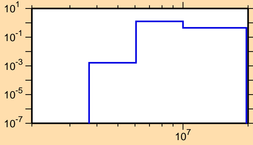
\sigma vs. E for ^{152}\text{Ho}(n,np)
