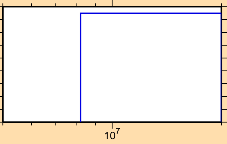
\sigma vs. E for ^{153}\text{Ho} (mt 42)
