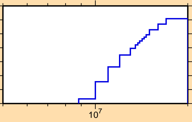
\sigma vs. E for ^{154}\text{Ho}(\text{mt117})
