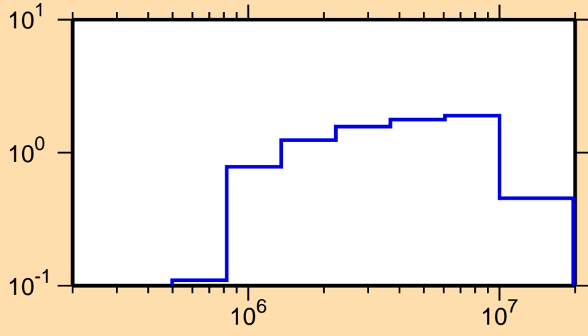
\sigma vs. E for ^{154}\text{Ho}(n,n\text{cont.})
