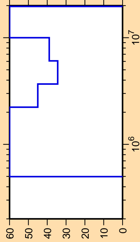
\Delta\sigma/\sigma vs. E for ^{154}\text{Ho}(n,n\text{cont.})
