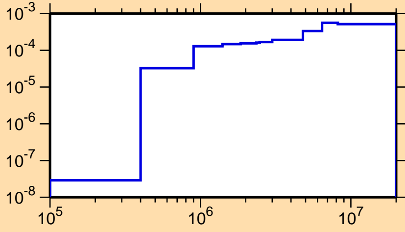
\sigma vs. E for ^{154}\text{Ho}(n,n_2)
