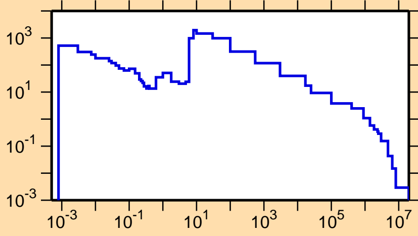
\sigma vs. E for ^{154}\text{Ho}(n,\gamma)
