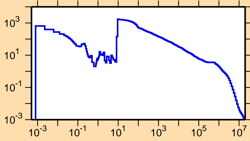
\sigma vs. E for ^{156}\text{Ho}(n,\gamma)
