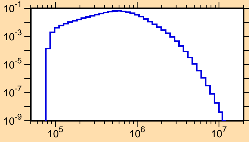
\sigma vs. E for ^{156}\text{Ho}(n,n_2)
