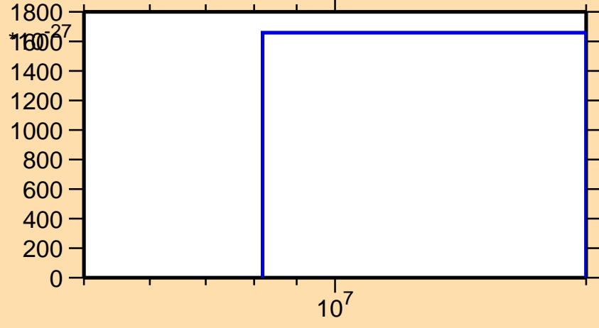
\sigma vs. E for ^{156}\text{Ho} (mt 42)
