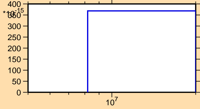
\sigma vs. E for ^{156}\text{Ho}(n,pd)
