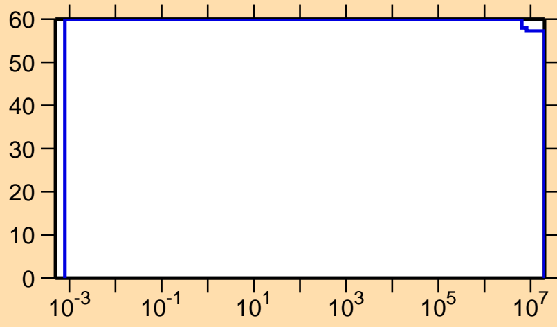
\Delta\sigma/\sigma vs. E for ^{156}\text{Ho}(n,p)
