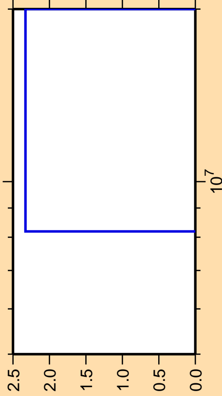
\Delta\sigma/\sigma vs. E for ^{156}\text{Ho}(n,pd)
