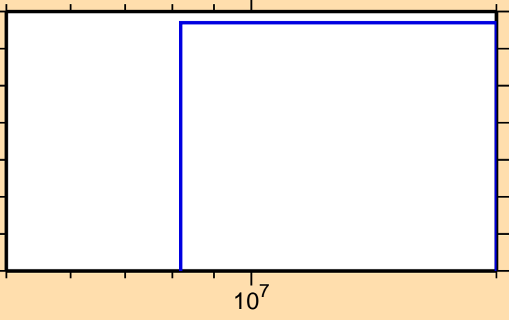
\sigma vs. E for ^{156}\text{Ho} (mt 45)
