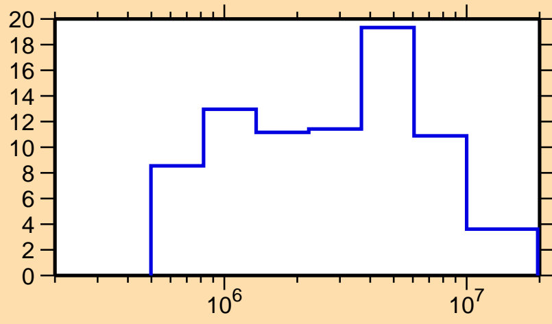
\Delta\sigma/\sigma vs. E for ^{156}\text{Ho}(n, el.)
