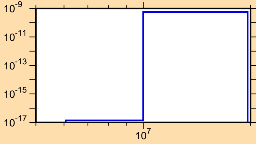
\sigma vs. E for ^{156}\text{Ho}(\text{mt117})
