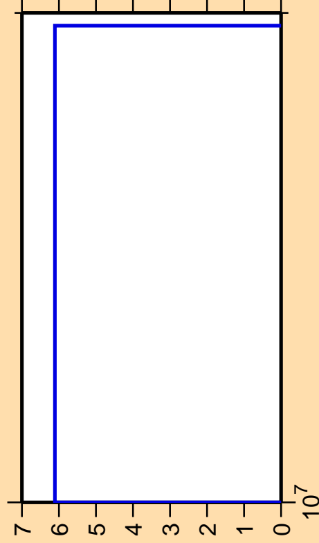
\Delta\sigma/\sigma vs. E for ^{156}\text{Ho} (mt 34)
