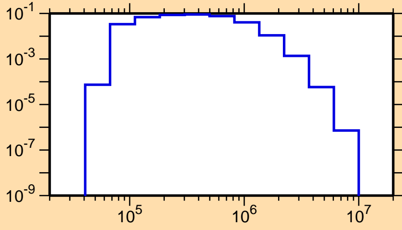
\sigma vs. E for ^{156}\text{Ho}(n,n_4)
