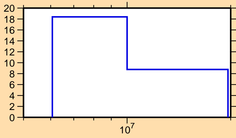
\Delta\sigma/\sigma vs. E for ^{156}\text{Ho}(n,2n)
