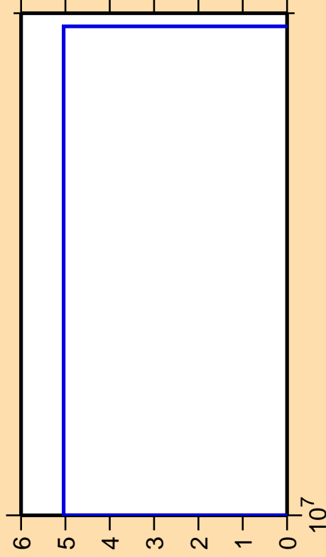
\Delta\sigma/\sigma vs. E for ^{156}\text{Ho}(n,\text{pt})
