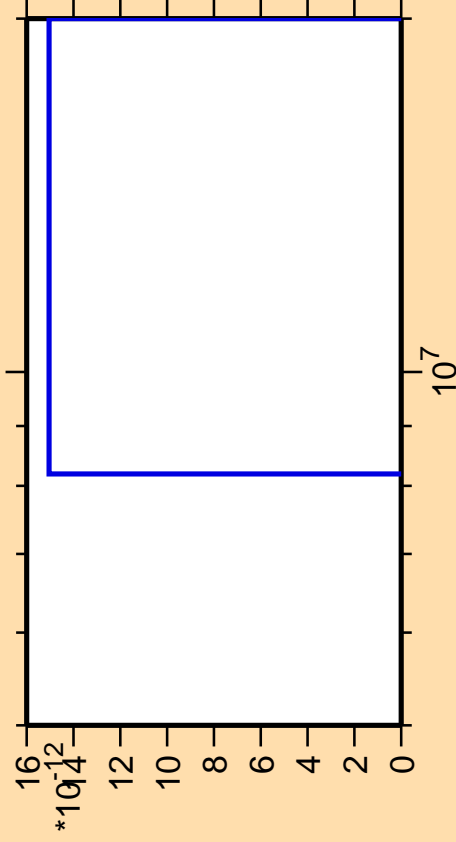
\Delta\sigma/\sigma vs. E for ^{156}\text{Ho} (mt 42)
