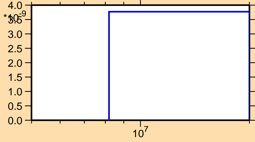
\sigma vs. E for ^{156}\text{Ho} (mt 45)
