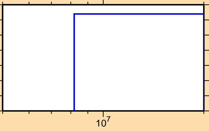
\sigma vs. E for ^{156}\text{Ho}(n,\text{nd})
