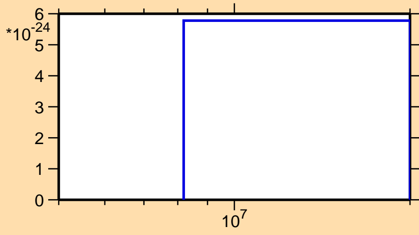
\sigma vs. E for ^{156}\text{Ho} (mt 42)
