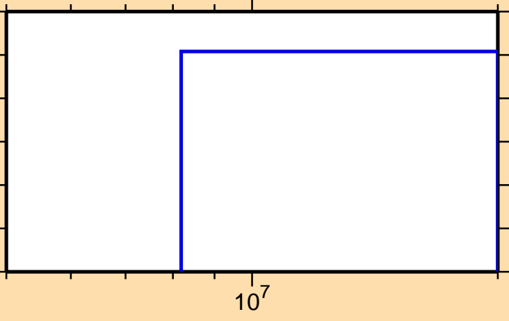
\sigma vs. E for ^{156}\text{Ho}(n,\text{pt})
