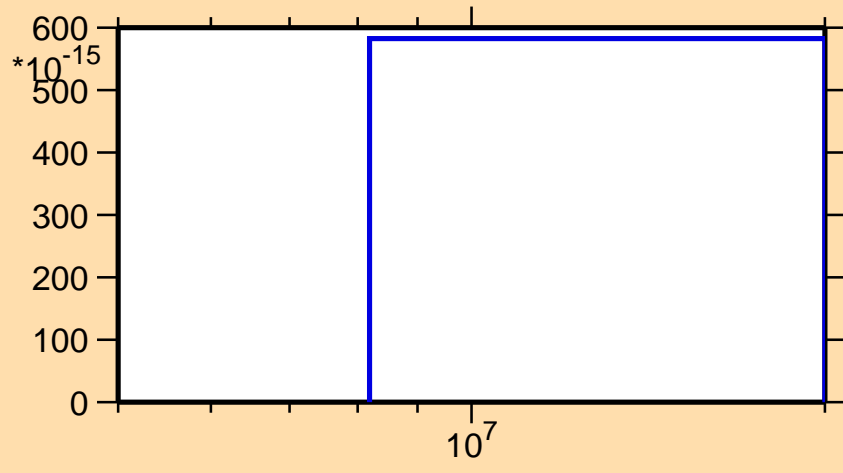
\sigma vs. E for ^{156}\text{Ho}(n,pd)
