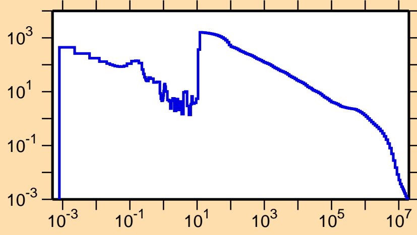
\sigma vs. E for ^{157}\text{Ho}(n,\gamma)
