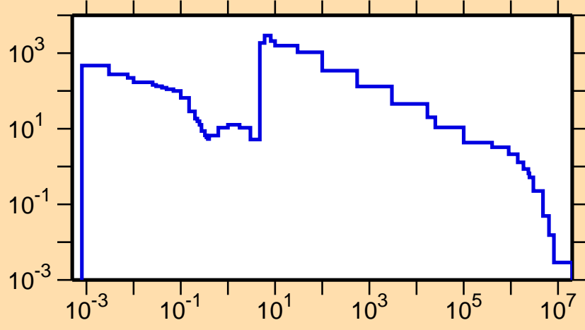
\sigma vs. E for ^{158}\text{Ho}(n,\gamma)
