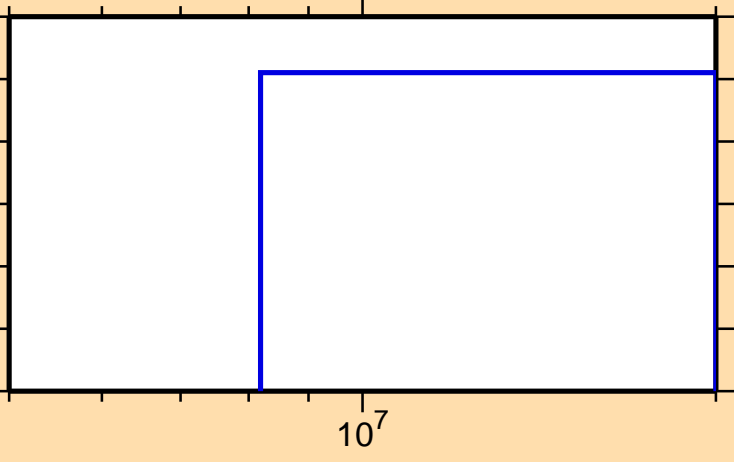
\sigma vs. E for ^{158}\text{Ho}(\text{mt117})
