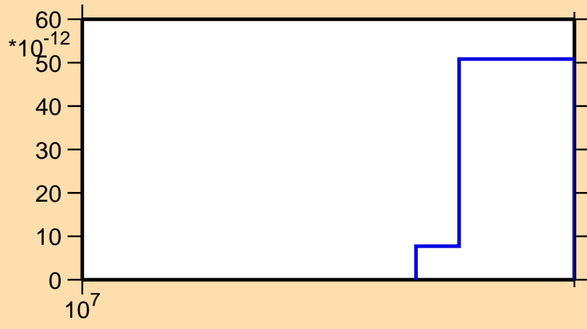
\sigma vs. E for ^{158}\text{Ho}(\text{mt117})
