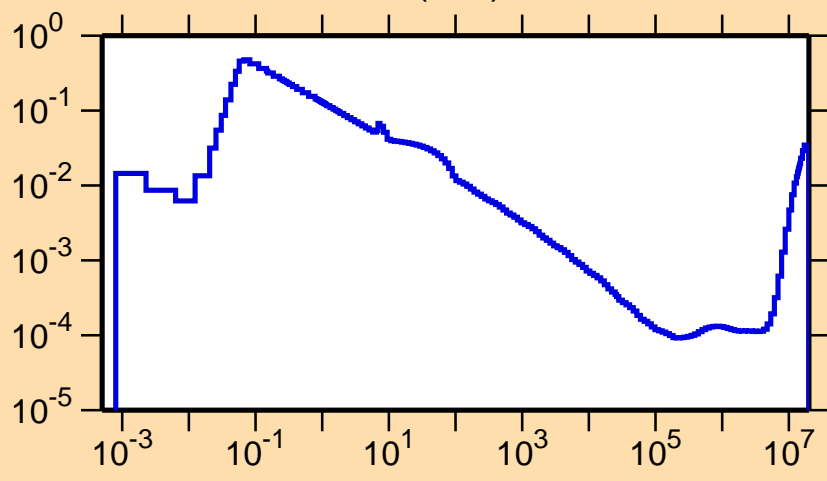
\sigma vs. E for ^{158}\text{Ho}(n,\alpha)
