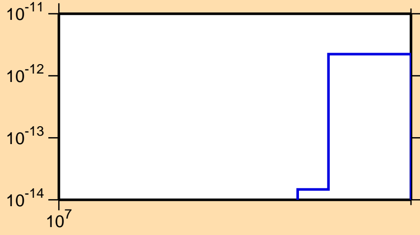
\sigma vs. E for ^{158}\text{Ho}(n,\text{pt})
