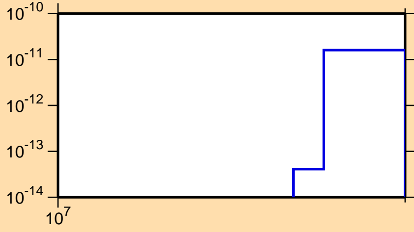
\sigma vs. E for ^{158}\text{Ho} (mt 34)
