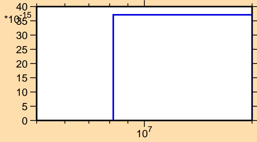
\sigma vs. E for ^{158}\text{Ho}(n,pd)
