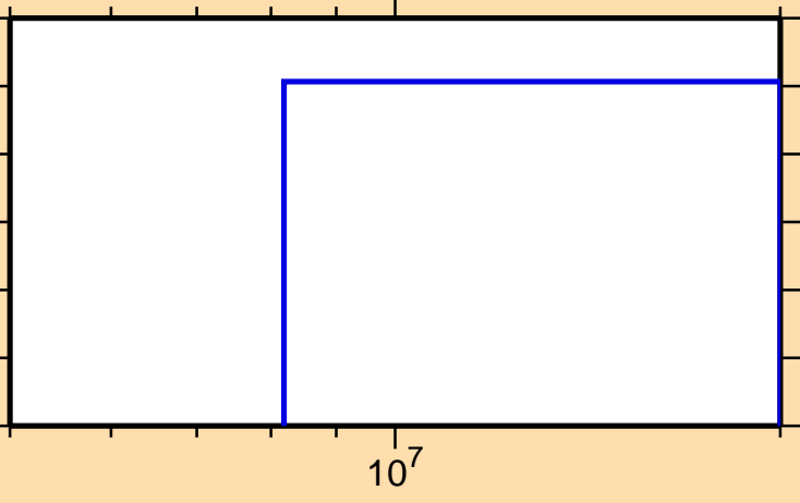
\sigma vs. E for ^{158}\text{Ho}(n,nt)
