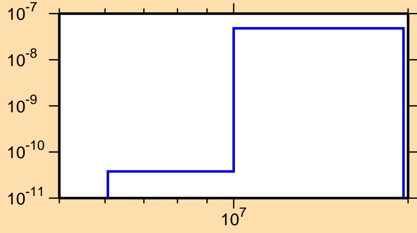
\sigma vs. E for ^{158}\text{Ho}(n,p\alpha)
