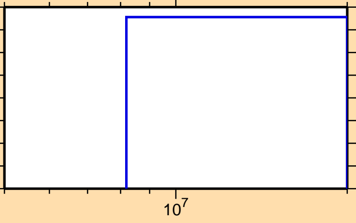
\sigma vs. E for ^{158}\text{Ho}(n,\text{pt})
