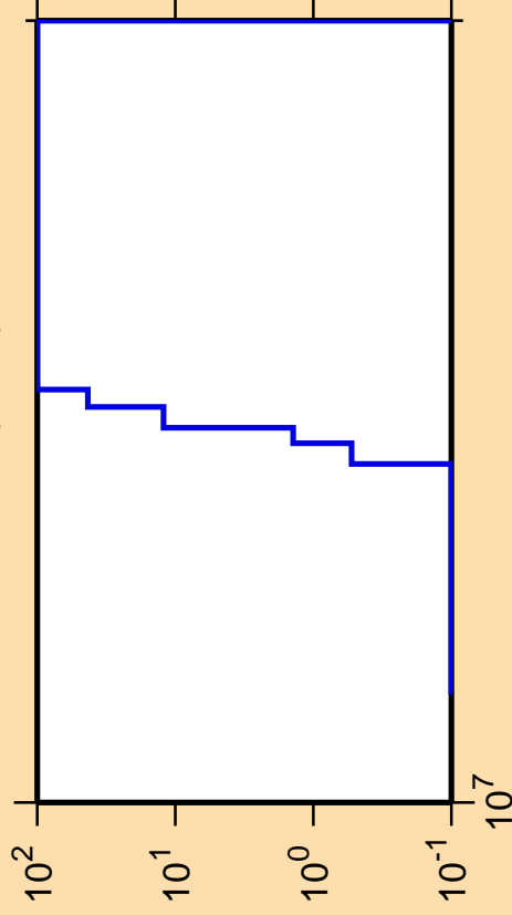
\Delta\sigma/\sigma vs. E for ^{159}\text{Ho}(n,\text{nd})
