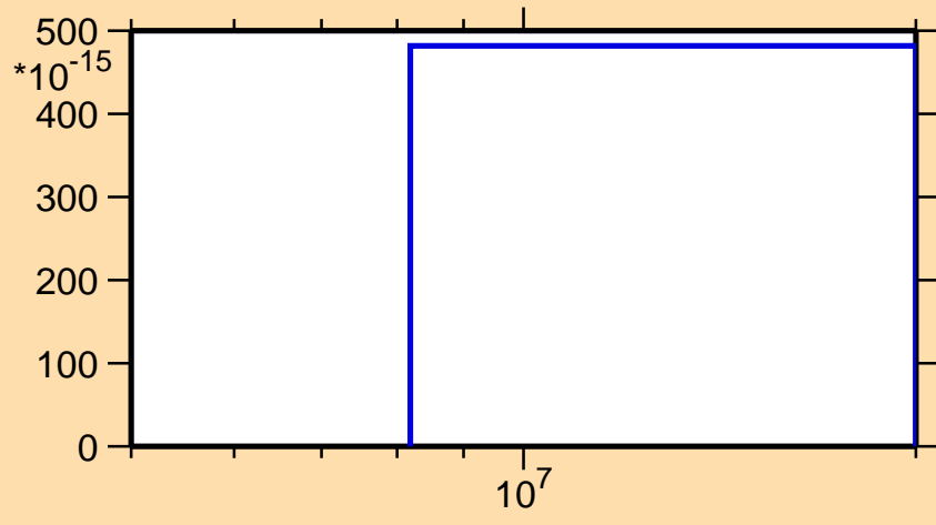
\sigma vs. E for ^{159}\text{Ho} (mt 45)
