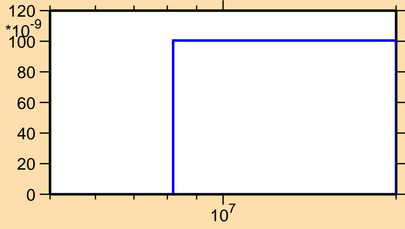
\sigma vs. E for ^{159}\text{Ho}(n,2np)
