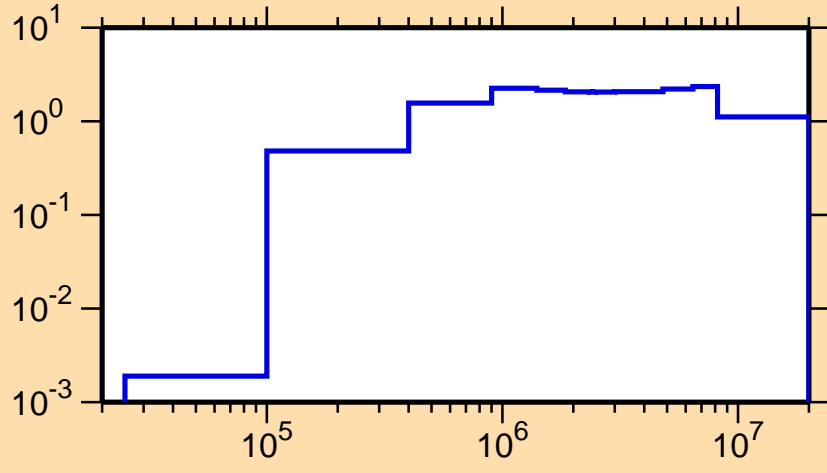
\sigma vs. E for ^{159}\text{Ho}(n,\text{inel.})
