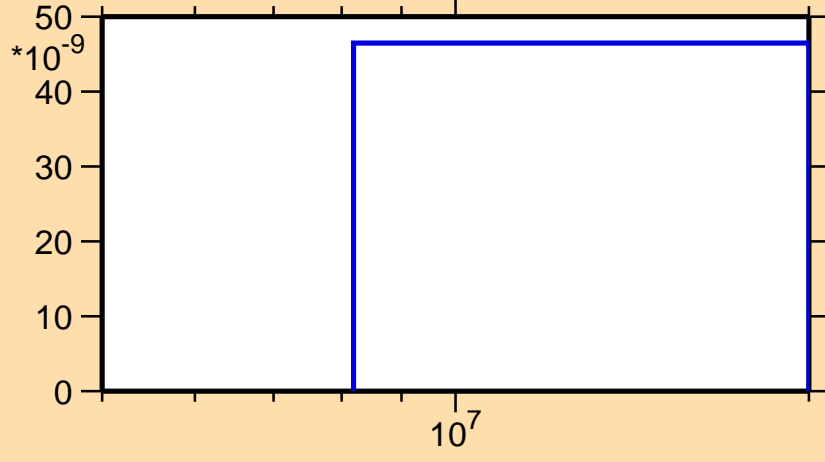
\sigma vs. E for ^{159}\text{Ho}(n,\text{nd})
