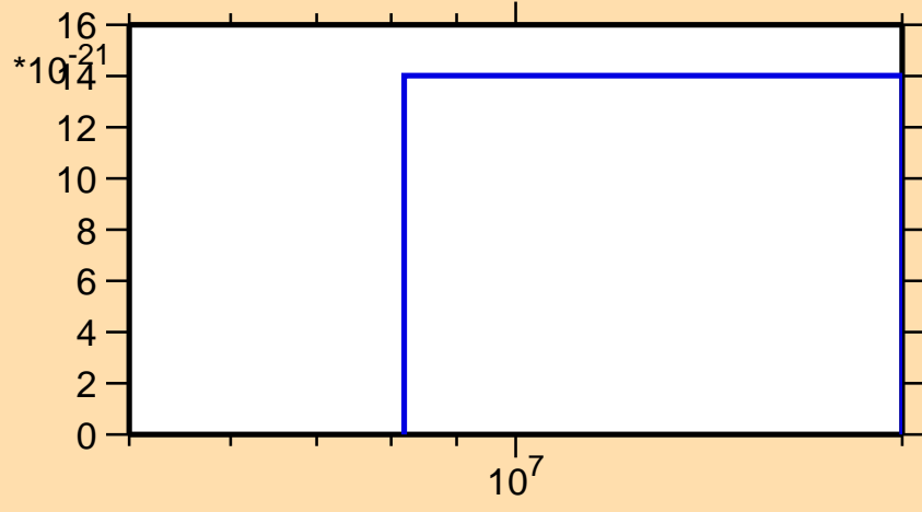
\sigma vs. E for ^{159}\text{Ho} (mt 11)
