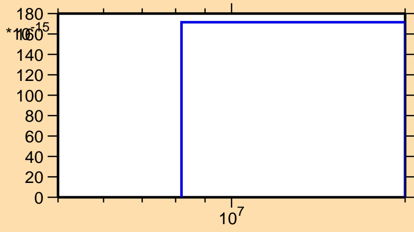
\sigma vs. E for ^{159}\text{Ho}(\text{mt117})
