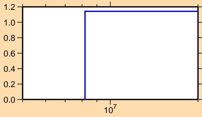
\sigma vs. E for ^{159}\text{Ho}(n,2n)
