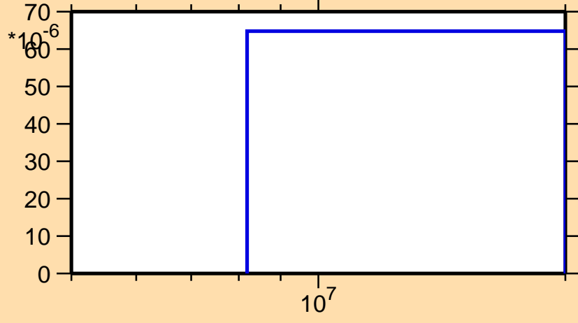
\sigma vs. E for ^{159}\text{Ho}(n,t)
