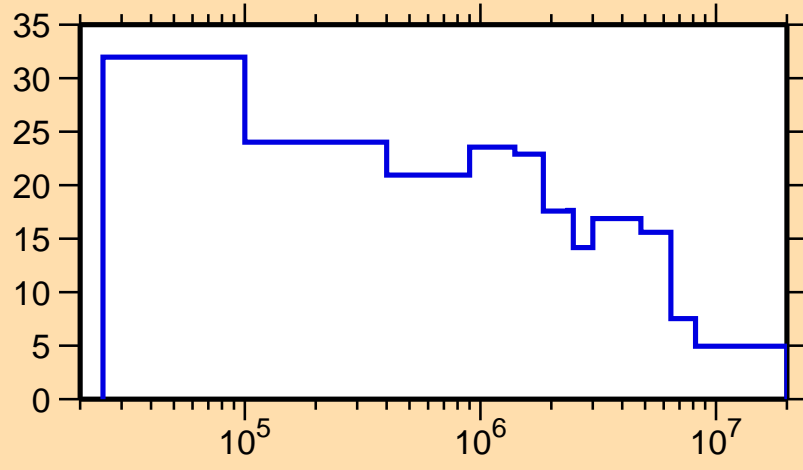
\Delta\sigma/\sigma vs. E for ^{159}\text{Ho}(n,\text{tot.})
