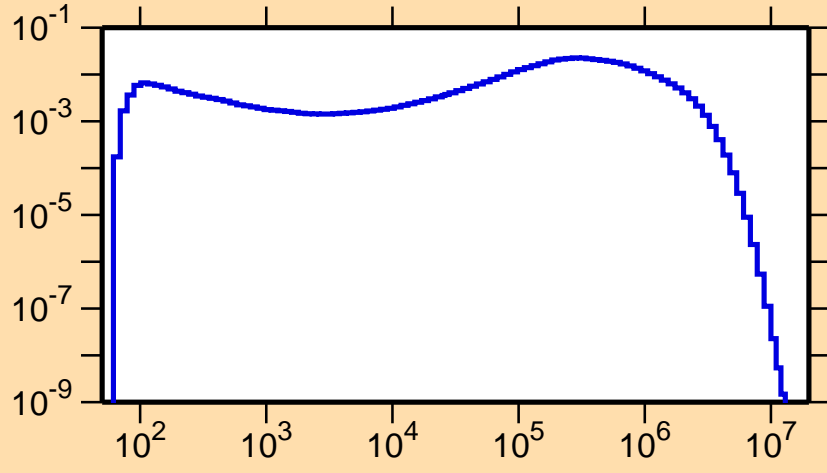
\sigma vs. E for ^{159}\text{Ho}(n,n_2)
