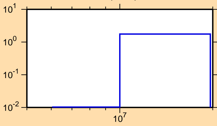
\sigma vs. E for ^{159}\text{Ho}(n,2n)
