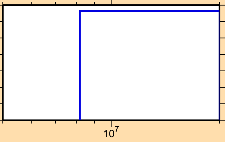
\sigma vs. E for ^{159}\text{Ho}(n,nt)
