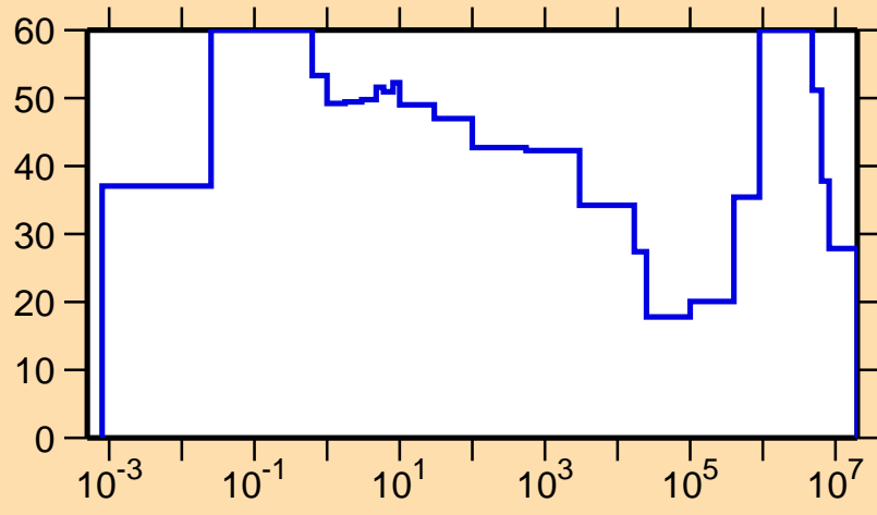
\Delta\sigma/\sigma vs. E for ^{159}\text{Ho}(n,p)
