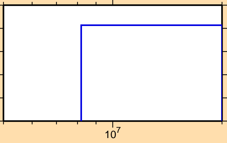
\sigma vs. E for ^{159}\text{Ho}(n,t)
