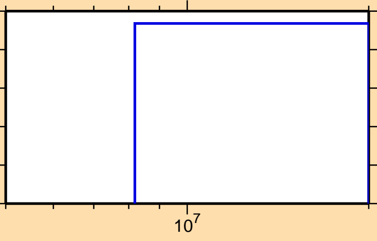
\sigma vs. E for ^{159}\text{Ho}(\text{mt117})
