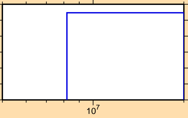
\sigma vs. E for ^{159}\text{Ho}(n,\text{nd})
