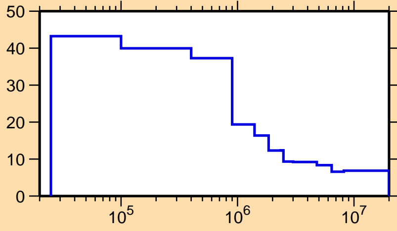
\Delta\sigma/\sigma vs. E for ^{160}\text{Ho}(n,\text{nonel.})
