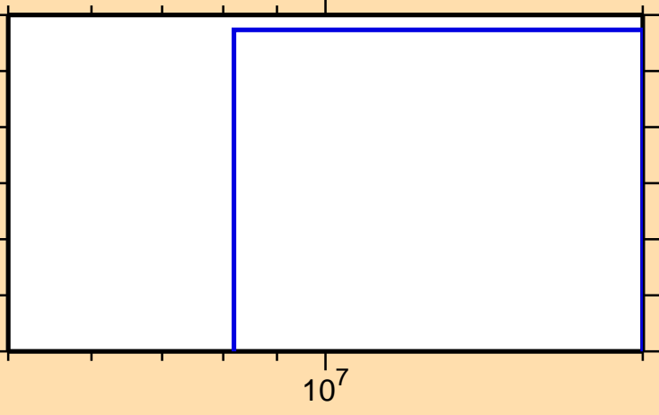
\sigma vs. E for ^{160}\text{Ho}(n,\text{pd})
