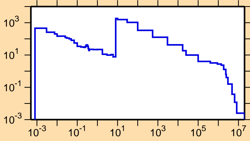
\sigma vs. E for ^{160}\text{Ho}(n,\gamma)
