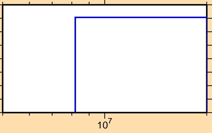
\sigma vs. E for ^{160}\text{Ho} (mt 45)
