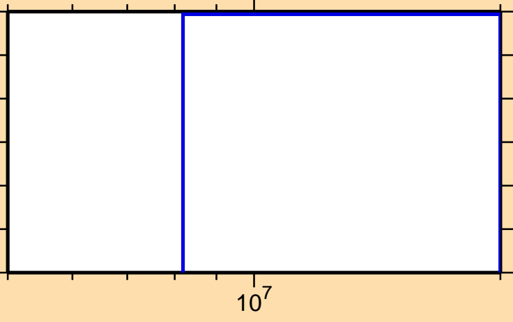
\sigma vs. E for ^{160}\text{Ho}(n,\text{He3})
