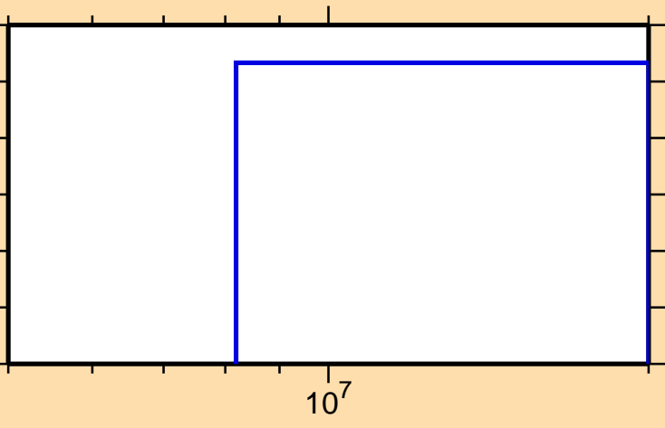
\sigma vs. E for ^{160}\text{Ho}(n,2n\alpha)
