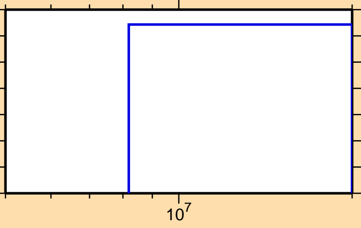
\sigma vs. E for ^{160}\text{Ho}(n,\text{He3})
