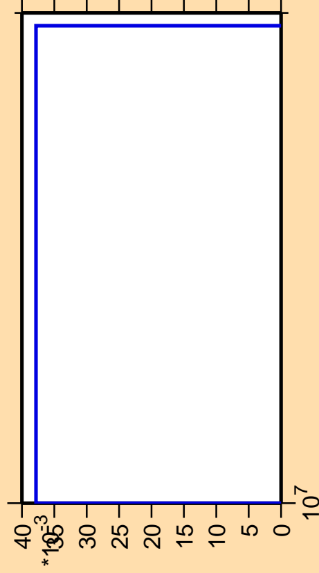
\Delta\sigma/\sigma vs. E for ^{161}\text{Ho} (mt 45)
