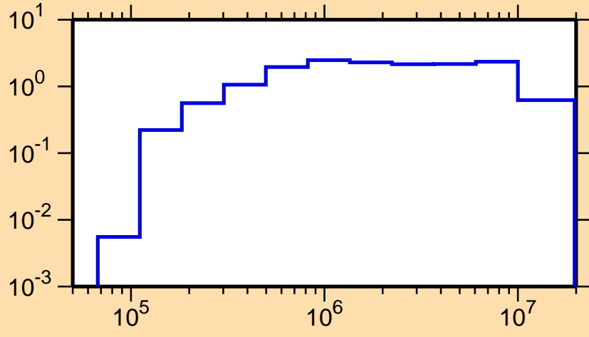
\sigma vs. E for ^{161}\text{Ho}(n,\text{inel.})
