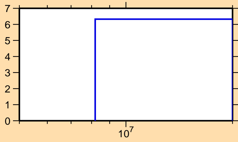
\Delta\sigma/\sigma vs. E for ^{161}\text{Ho}(n,\text{nonel.})
