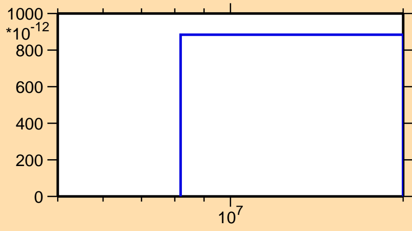
\sigma vs. E for ^{161}\text{Ho}(n,2n\alpha)
