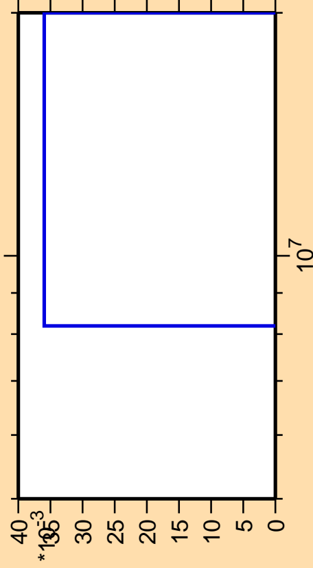
\Delta\sigma/\sigma vs. E for ^{161}\text{Ho}(\text{mt117})
