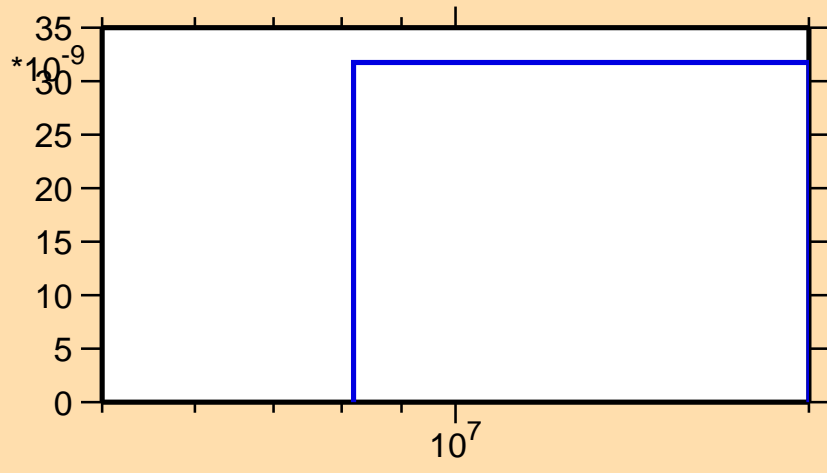
\sigma vs. E for ^{161}\text{Ho}(n,2np)
