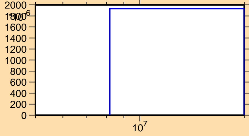
\sigma vs. E for ^{161}\text{Ho}(n,3n)
