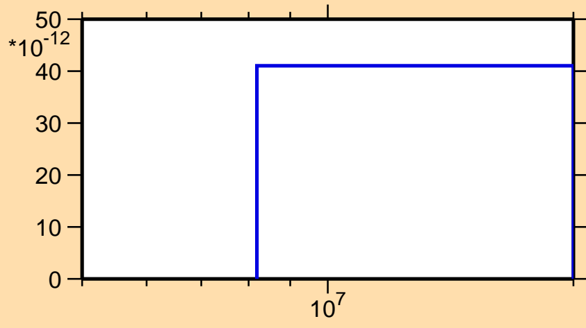
\sigma vs. E for ^{161}\text{Ho}(n,p\alpha)
