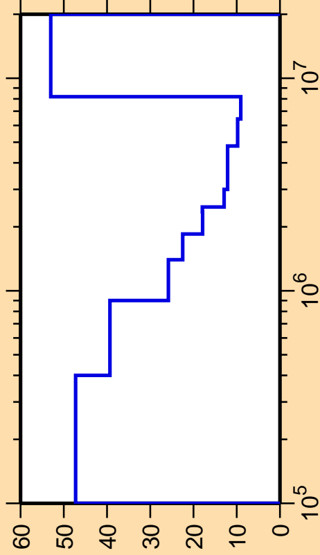
\Delta\sigma/\sigma vs. E for ^{161}\text{Ho}(n,\text{inel.})
