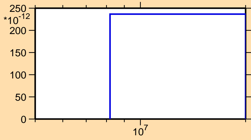
\sigma vs. E for ^{161}\text{Ho}(n,\text{He3})
