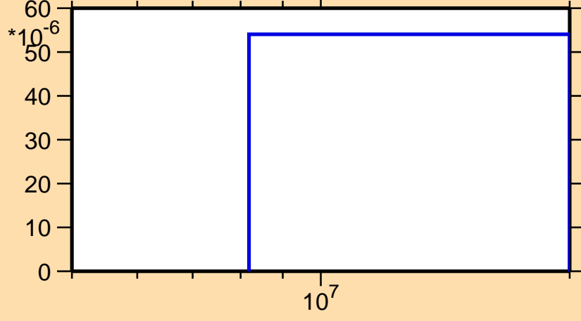
\sigma vs. E for ^{161}\text{Ho}(n,t)
