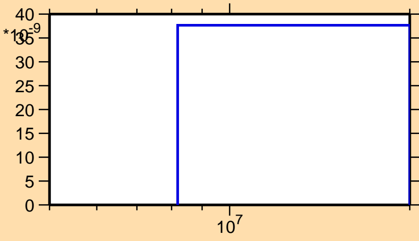
\sigma vs. E for ^{161}\text{Ho}(n,\text{nd})
