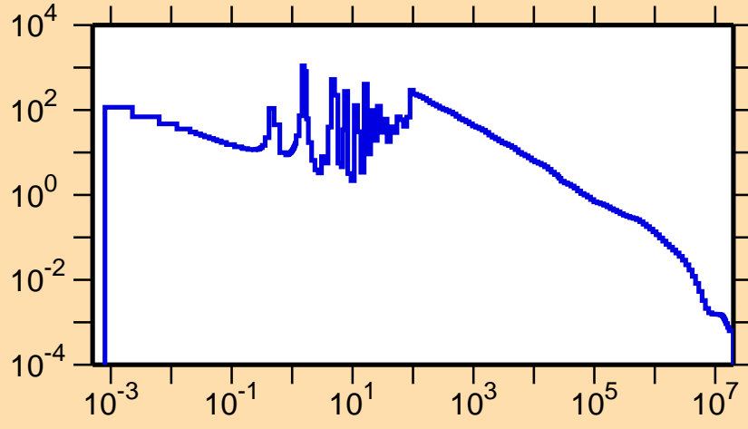
\sigma vs. E for ^{161}\text{Ho}(n,\gamma)
