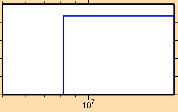
\sigma vs. E for ^{161}\text{Ho}(n,\text{nd})
