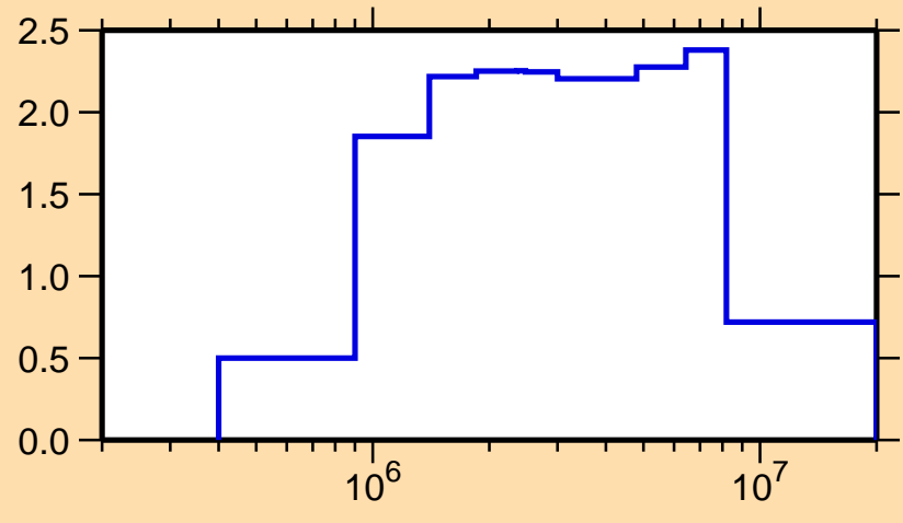
\sigma vs. E for ^{161}\text{Ho}(n,n\text{cont.})
