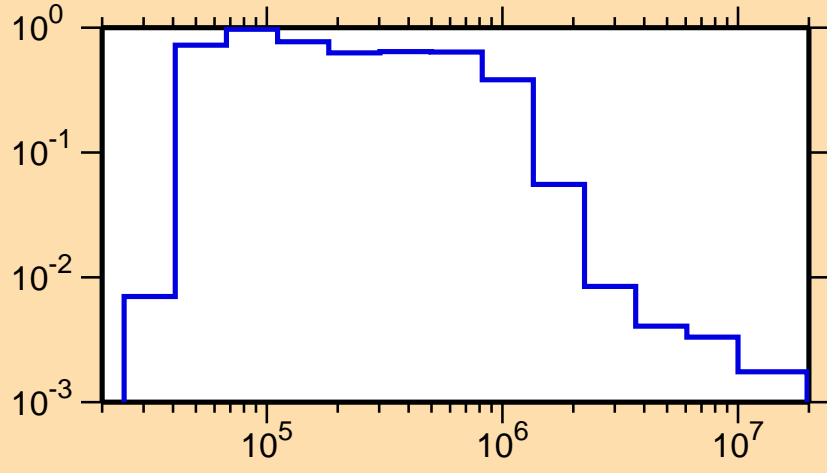
\sigma vs. E for ^{162}\text{Ho}(n,n_1)
