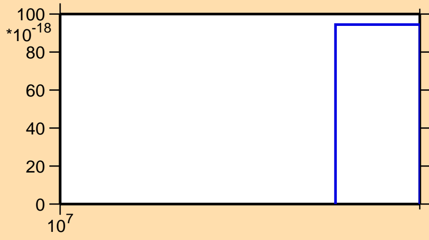
\sigma vs. E for ^{162}\text{Ho} (mt 11)
