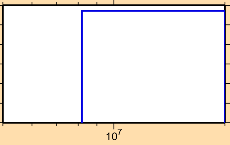
\sigma vs. E for ^{162}\text{Ho} (mt 34)
