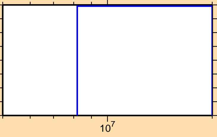
\sigma vs. E for ^{162}\text{Ho}(n,3n)
