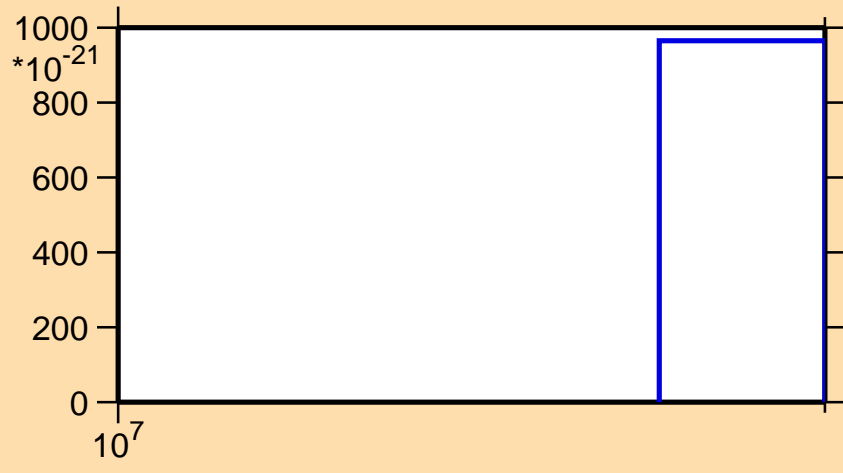
\sigma vs. E for ^{163}\text{Ho} (mt 11)
