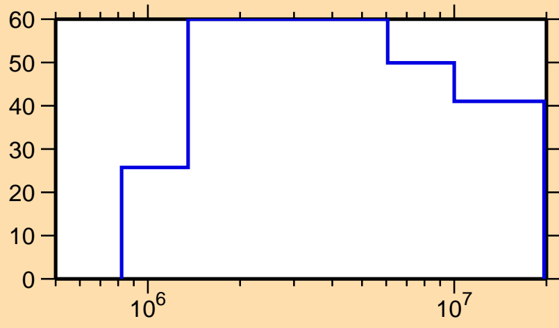
\Delta\sigma/\sigma vs. E for ^{163}\text{Ho}(n,p)
