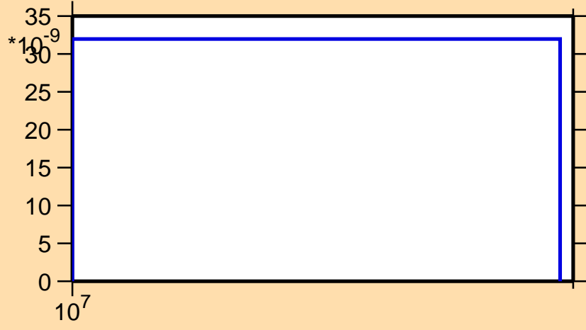
\sigma vs. E for ^{163}\text{Ho}(n,\text{nd})
