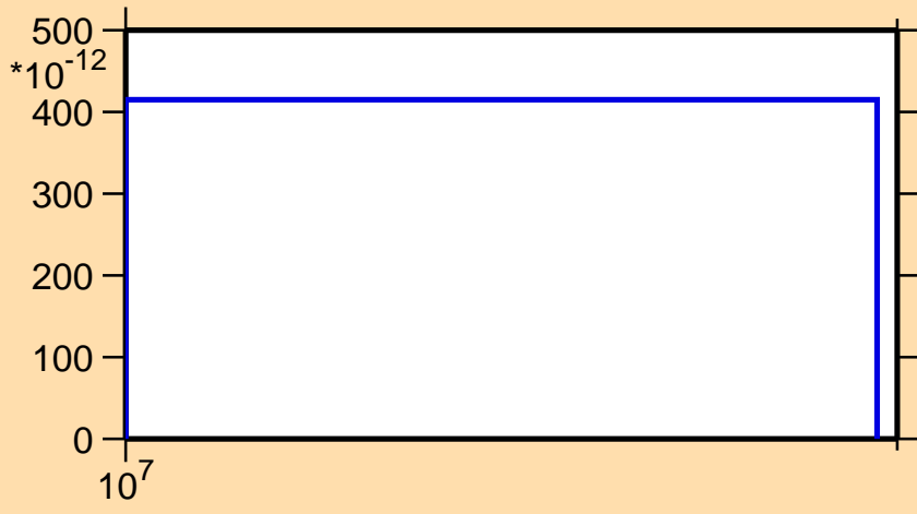
\sigma vs. E for ^{163}\text{Ho}(n,2n\alpha)
