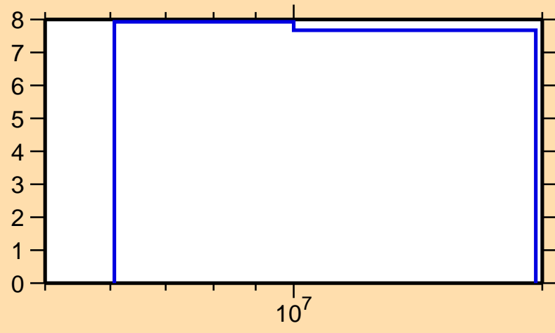
\Delta\sigma/\sigma vs. E for ^{163}\text{Ho}(n,\text{nonel.})
