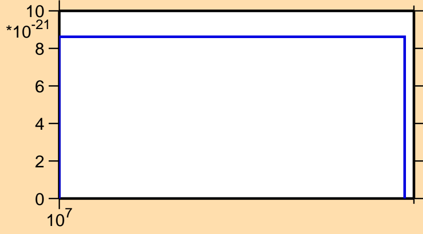
\sigma vs. E for ^{163}\text{Ho} (mt 11)
