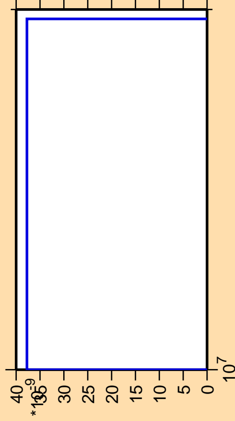
\Delta\sigma/\sigma vs. E for ^{163}\text{Ho} (mt 11)
