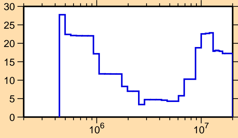
\Delta\sigma/\sigma vs. E for ^{163}\text{Ho}(n,n\text{cont.})
