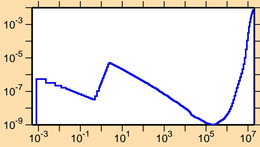
\sigma vs. E for ^{163}\text{Ho}(n,\alpha)
