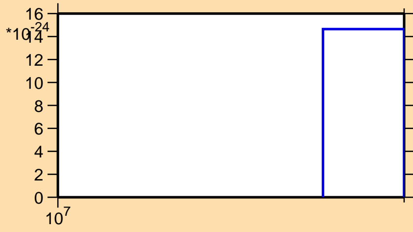
\sigma vs. E for ^{163}\text{Ho} (mt 42)
