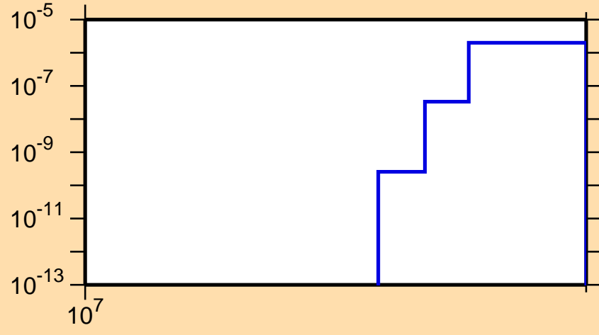
\sigma vs. E for ^{163}\text{Ho}(n,2np)
