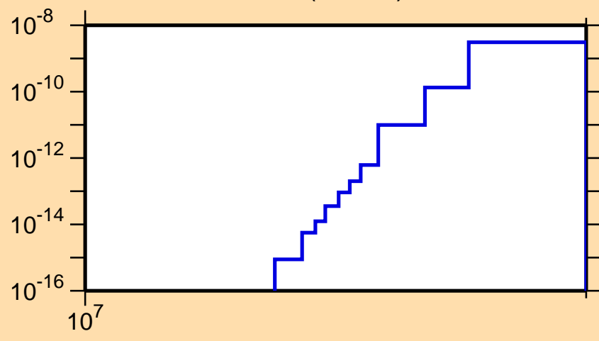
\sigma vs. E for ^{163}\text{Ho}(n,\text{He3})
