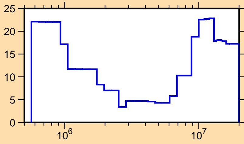
\Delta\sigma/\sigma vs. E for ^{163}\text{Ho}(n,n\text{cont.})
