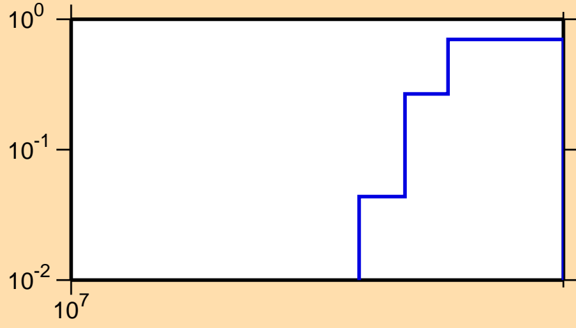
\sigma vs. E for ^{163}\text{Ho}(n,3n)
