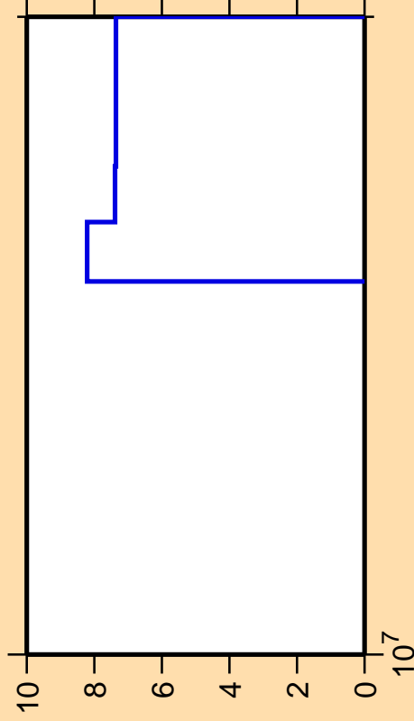
\Delta\sigma/\sigma vs. E for ^{163}\text{Ho}(n,3n)
