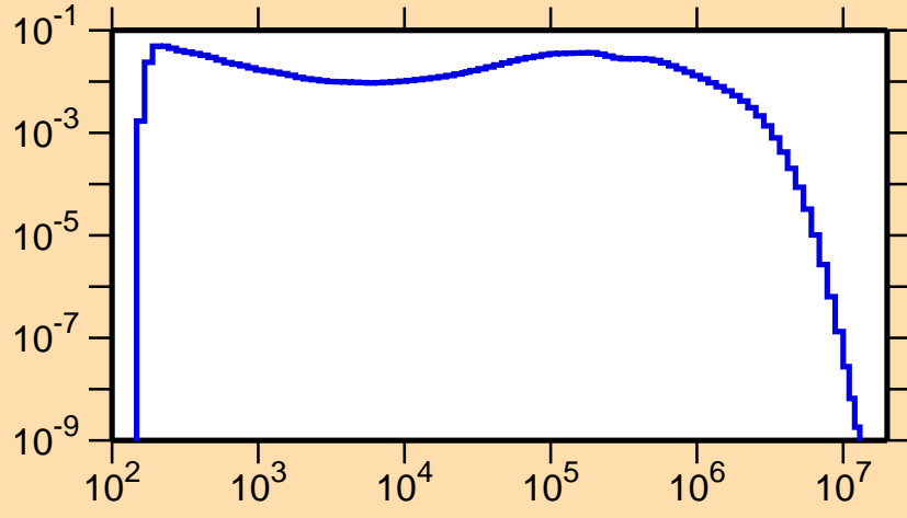
\sigma vs. E for ^{163}\text{Ho}(n,n_2)
