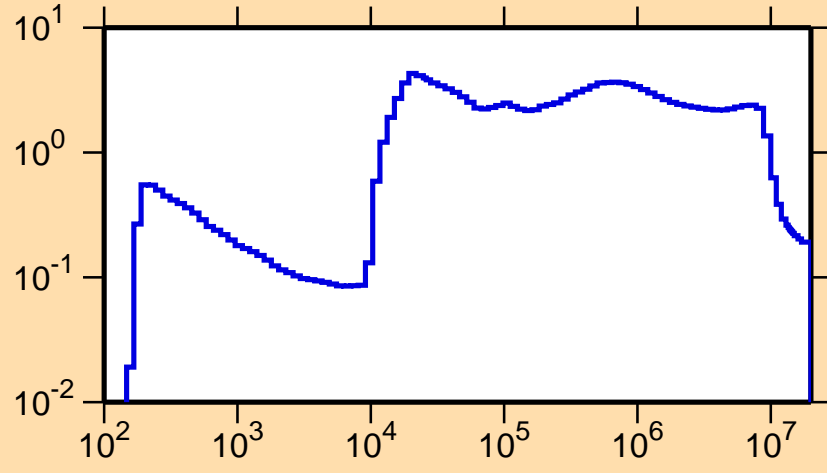
\sigma vs. E for ^{163}\text{Ho}(n,\text{inel.})
