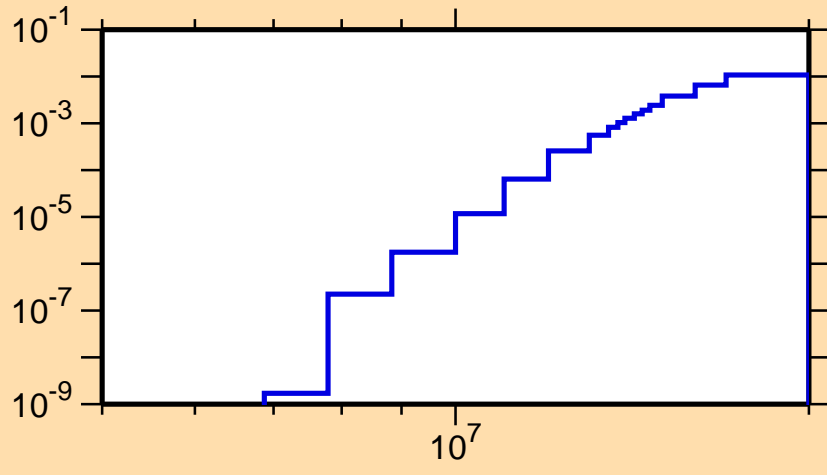
\sigma vs. E for ^{163}\text{Ho}(n,np)
