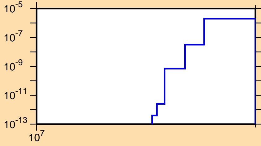
\sigma vs. E for ^{163}\text{Ho}(n,nt)
