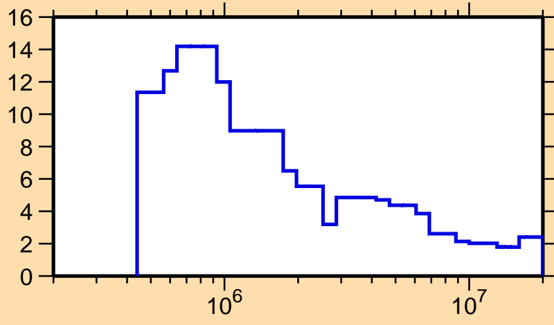
\Delta\sigma/\sigma vs. E for ^{163}\text{Ho}(n,\text{nonel.})
