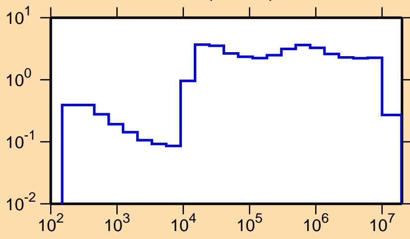
\sigma vs. E for ^{163}\text{Ho}(n,\text{inel.})
