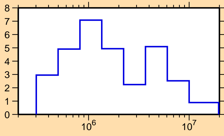
\Delta\sigma/\sigma vs. E for ^{163}\text{Ho}(n,\text{tot.})
