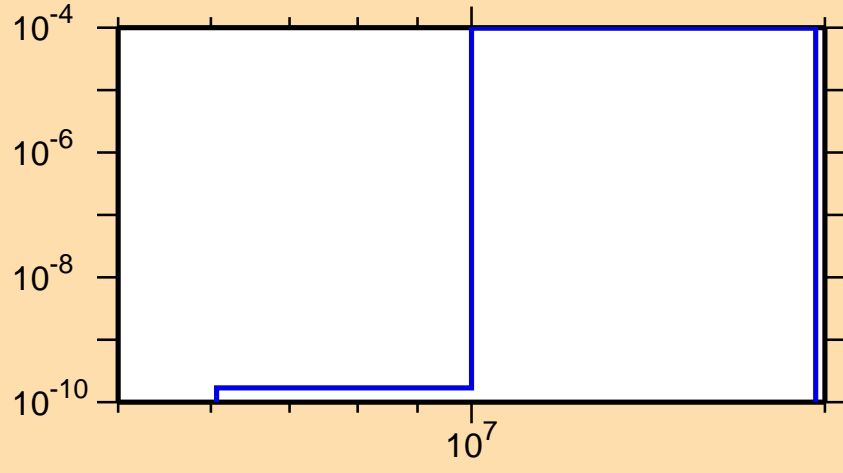
\sigma vs. E for ^{164}\text{Ho}(n,t)
