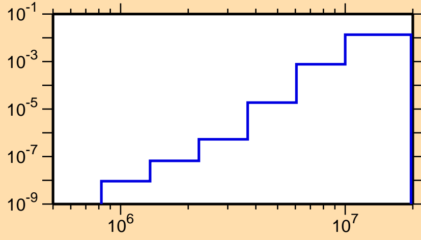
\sigma vs. E for ^{164}\text{Ho}(n,p)
