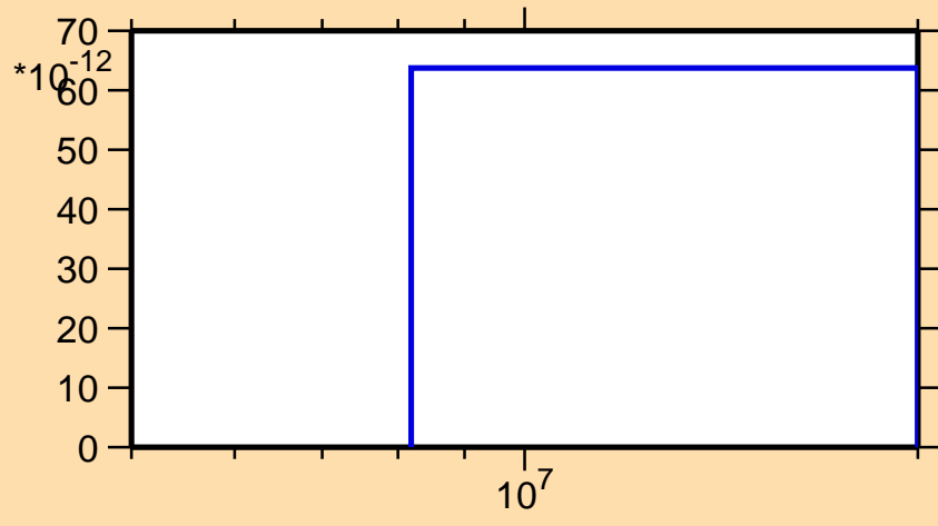
\sigma vs. E for ^{164}\text{Ho}(n,\text{He3})
