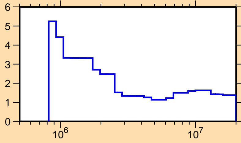
\Delta\sigma/\sigma vs. E for ^{165}\text{Ho}(n,n\text{onel.})
