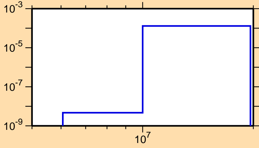
\sigma vs. E for ^{165}\text{Ho}(n,n\alpha)
