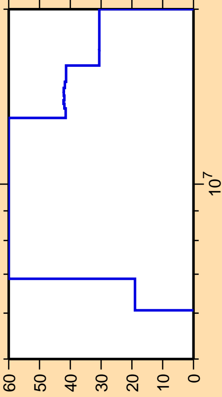
\Delta\sigma/\sigma vs. E for ^{166}\text{Ho}(n,n\text{cont.})
