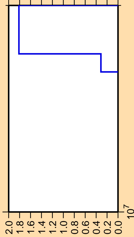
\Delta\sigma/\sigma vs. E for ^{166}\text{Ho}(n,p\alpha)
