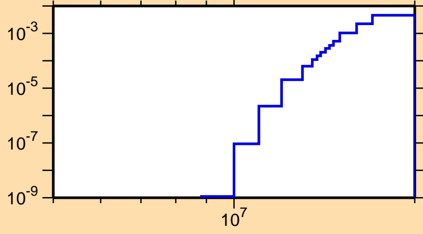
\sigma vs. E for ^{166}\text{Ho}(n,np)
