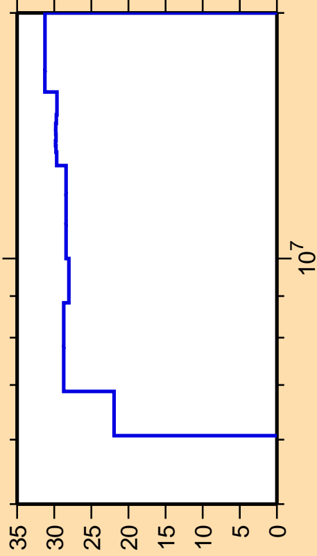
\Delta\sigma/\sigma vs. E for ^{166}\text{Ho}(n,n_1)
