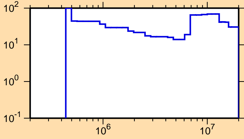
\Delta\sigma/\sigma vs. E for ^{166}\text{Ho}(n,n\text{cont.})
