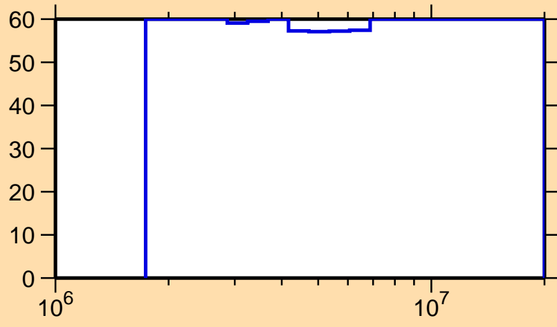
\Delta\sigma/\sigma vs. E for ^{166}\text{Ho}(n,\gamma)
