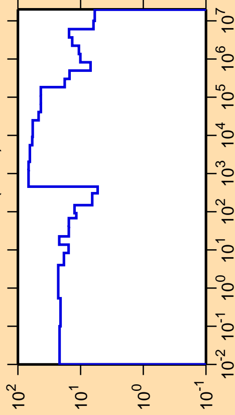
\Delta\sigma/\sigma vs. E for ^{166}\text{Ho}(n,\text{el.})
