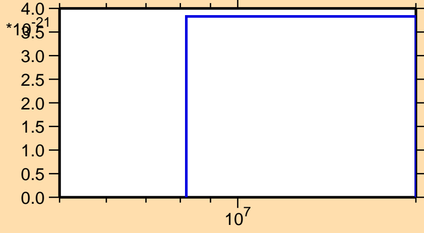
\sigma vs. E for ^{166}\text{Ho} (mt 11)
