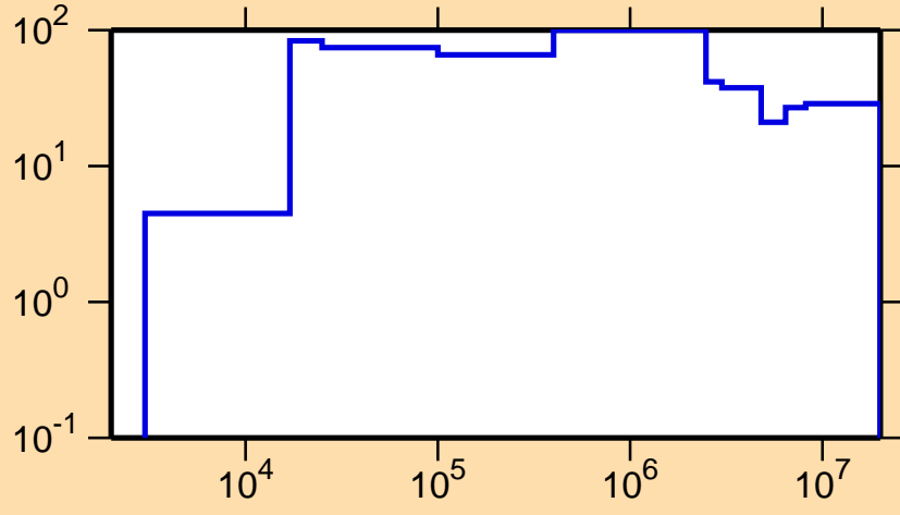
\Delta\sigma/\sigma vs. E for ^{166}\text{Ho}(n,n_1)
