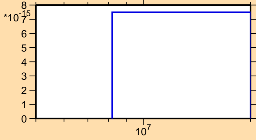
\sigma vs. E for ^{166}\text{Ho}(n,p\alpha)
