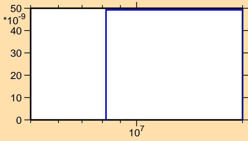
\sigma vs. E for ^{166}\text{Ho}(n,2np)
