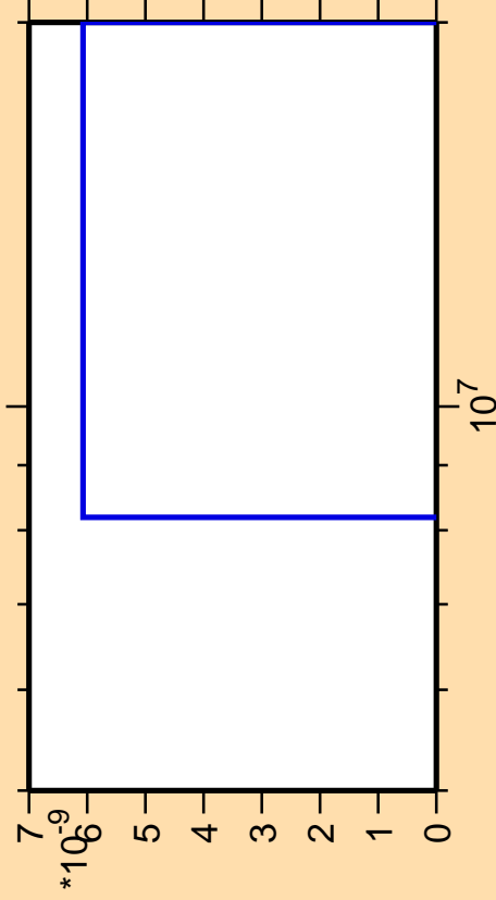
\Delta\sigma/\sigma vs. E for ^{166}\text{Ho} (mt 11)
