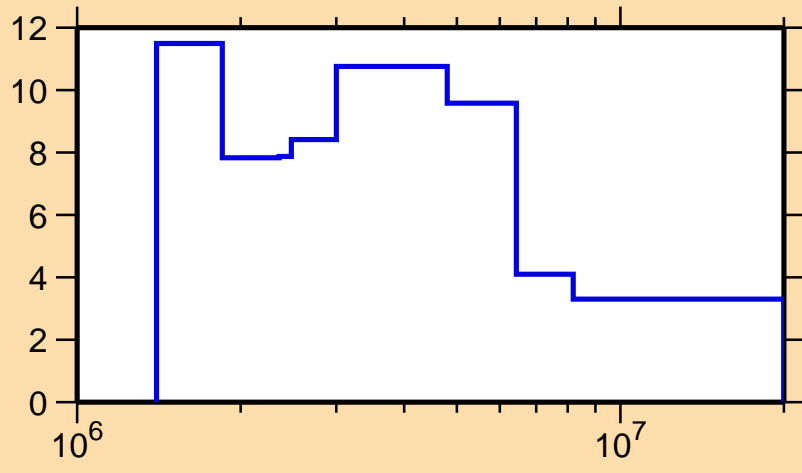
\Delta\sigma/\sigma vs. E for ^{166}\text{Ho}(n,\text{tot.})
