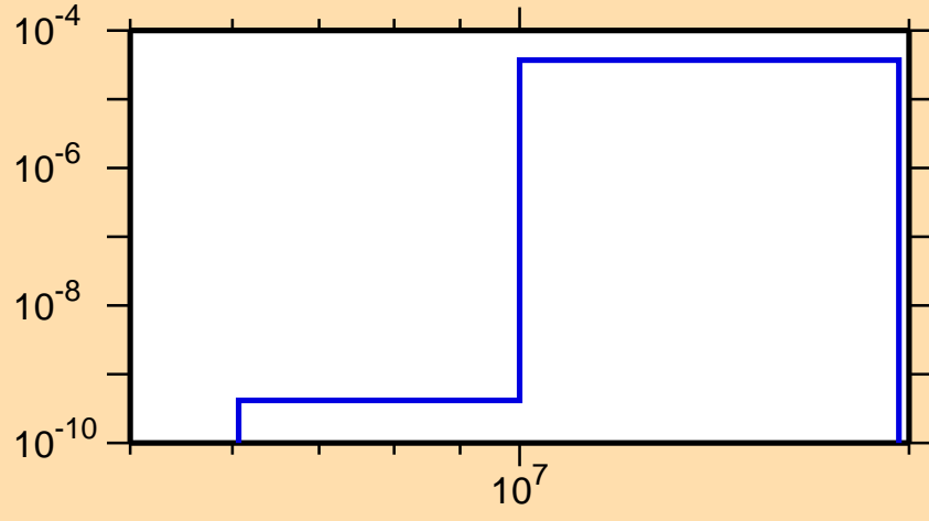
\sigma vs. E for ^{166}\text{Ho}(n,n\alpha)
